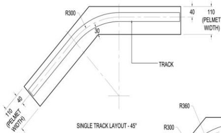
SINGLE TRACK LAYOUT - 45°
